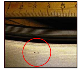
Pittings on outer race way
